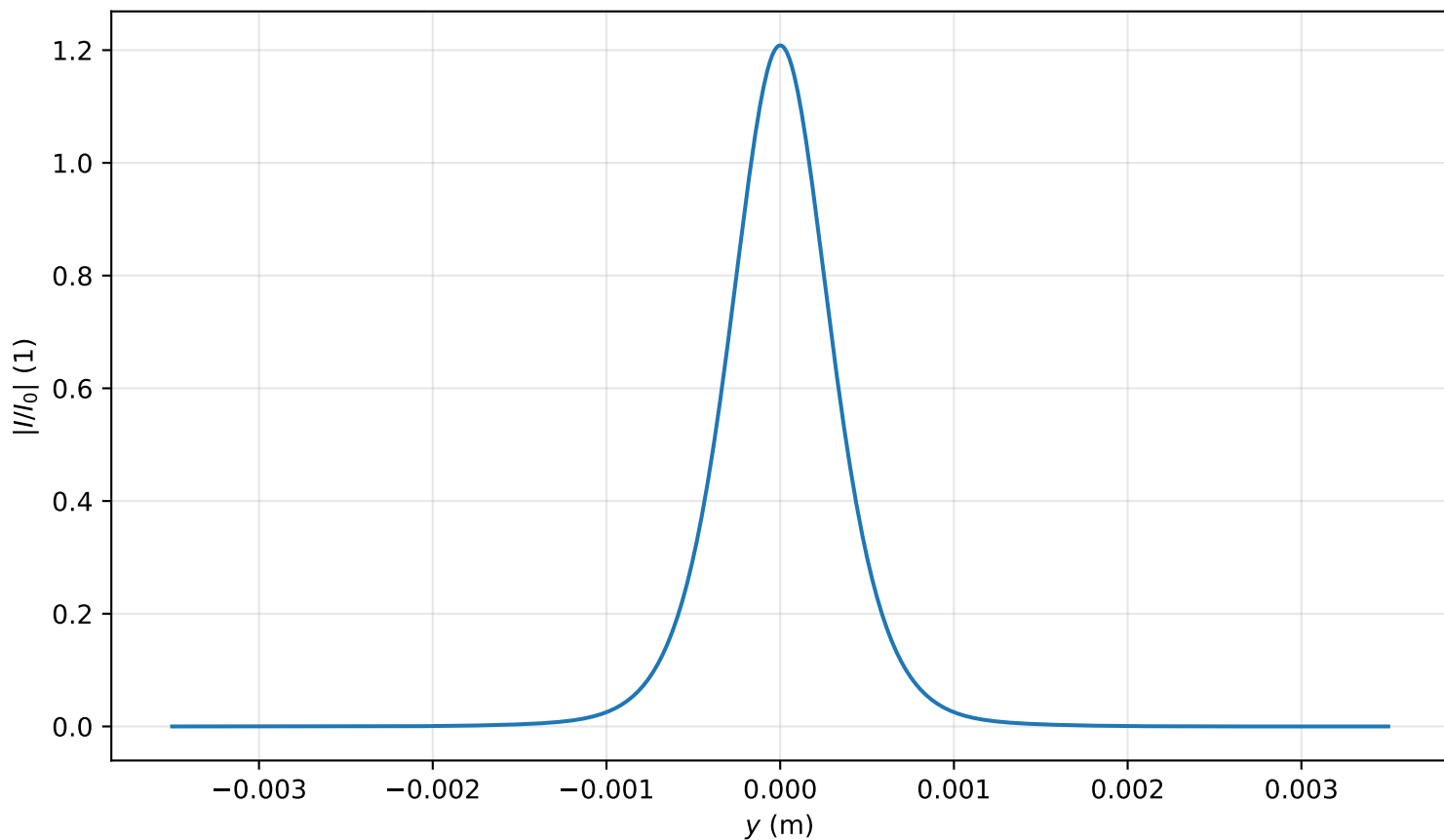
Intensity profile I(x=0, y, z=2.548)/I_0 , P_{in}=0.8P_{cr} , artificial time
